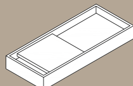
lavabo wash basin 120x50x15 cm 100 kg peso weight
