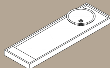
lavabo wash basin 180x50x10 cm 140 kg peso weight
